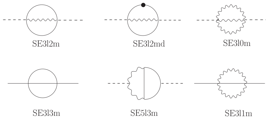
Figure 1: The six two-loop 2-point masters of Bhabha scattering.
