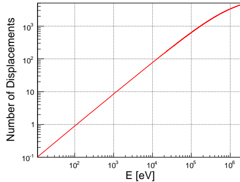
Figure 4: Number displaced atoms by ^{48}\text{Ti} recoils in Ti6Al4V target as function of ^{48}\text{Ti} energy.
