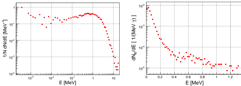
Figure 1: Energy distribution of neutrons (left) and recoil nuclei (right) in the Ti-alloy target.
