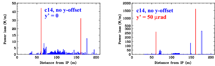
Figure 6: Beam loss in option c14 with solenoid, without (left) and with (right) 50 \mu rad y-orbit angle at IP.
