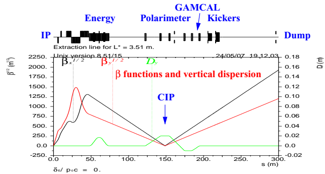
Figure 2: Extraction lattice functions.
