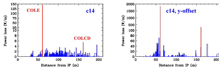
Figure 5: Beam loss in option c14 without (left) and with (right) IP y-offset for L^* = 3.51 m without solenoid.
