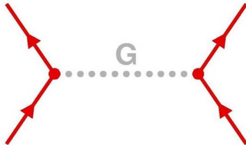
Gravitation
